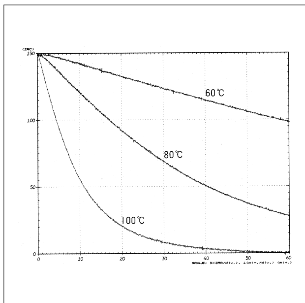
Fig. 2.22.6 Time course curves of the epoxy group at each temperature
