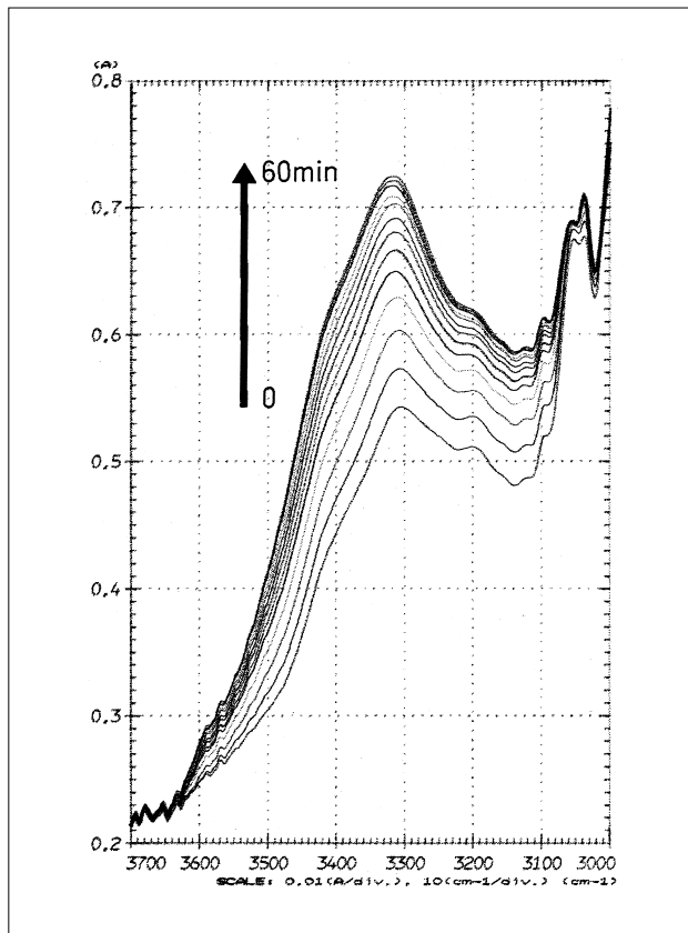
Fig. 2.22.4 Infrared spectra of the hydroxyl group
